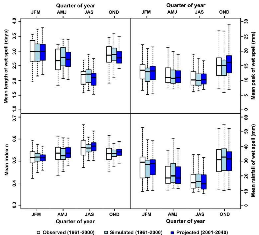
Fig. 9 Comparison of observed and simulated wet spells for 1961–2000 and those projected for 2001–2040. Each point of the boxplot represents the climatic value of a real or simulated station. The top left shows the average length of spells (days); the top right shows the average daily peak (in millimetres). The bottom right shows the average total rainfall (in millimetres) and the lower left compares the mean index n of the wet spell
