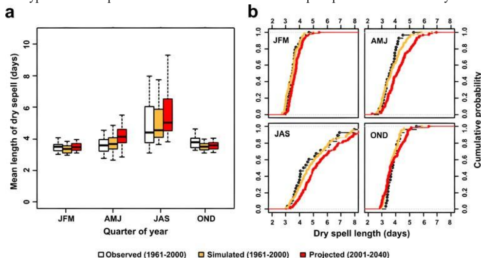
Fig. 10 Evolution of dry spells for the period of 2001–2040 versus the period 1961–2000, both observed and simulated: a boxplot of the average length of dry spells and b cumulative probability of the length of dry spells
