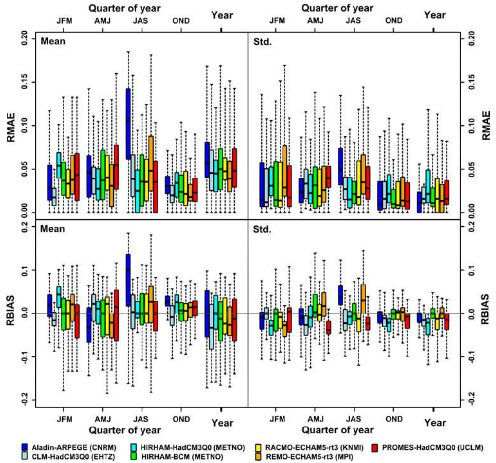
Fig. 3 Relative mean absolute error (RMAE) and relative bias (RBIAS) of the average and standard deviations of simulated time series. Each bar represents the set of all stations according to each of the seven RCMs
