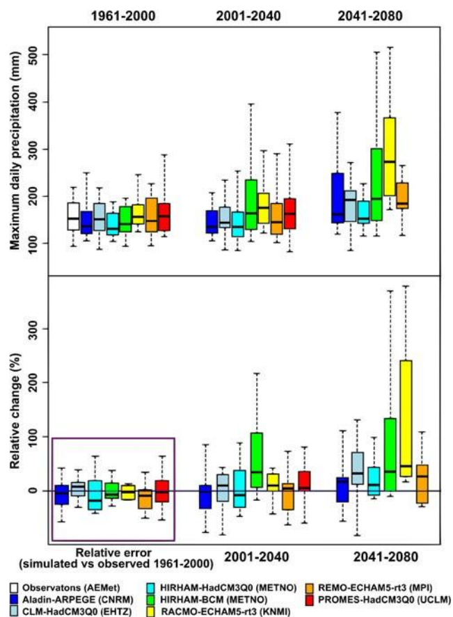
Fig. 6 Projection of the expected daily rainfall for a return period of 100 years according to the theoretical curves fitted to the simulated stations. The top shows the projection of the absolute value for the three periods (1961–2000, 2001–2040 and 2041–2080). The bottom shows the relative change for 2001–2040 and 2041–2080 and the error of the simulation compared with observed time series (1961–2000)
