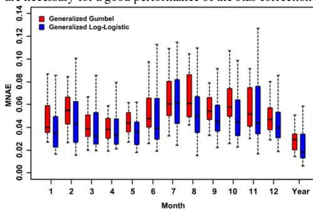
Fig. 2 Comparison of mean normalised absolute error (MNAE) of the two probabilistic models used for the standardisation of the 45 stations with at least 40 years of data
