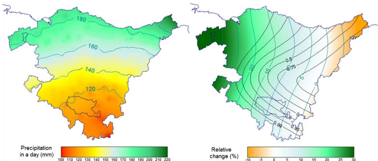
Fig. 7 Maximum expected rainfall in 1 day for 1961–2000 simulated shows the relative change of precipitation described at the left for the with a return period of 100 years (left). The values are estimated period 2001–2040 versus 1961–2000. The black lines represent the according to the theoretical curves fitted to the simulated stations, and confidence intervals estimated from the statistics of the seven RCMs they are interpolated by using a multiple spatial fit. The image at the right
