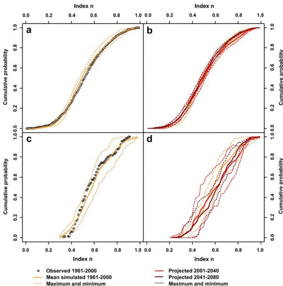
Fig. 8 a Empirical probability distribution of the index n to the set of all the stations in the period 1961–2000 and the range corresponding to the seven RCM simulations. b Projection of change for 2001–2040 and 2041–2080. c, d Respectively the same as a and b but only the rainfall exceeded 50 mm in 1 day
