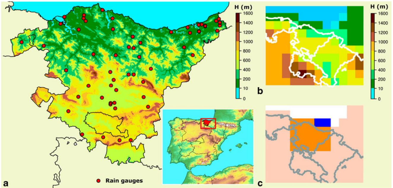
Fig. 1 a Location of the stations used in this study (AEMET). b Example of digital terrain model used in the regional climate models of ENSEMBLESr3. c Election of interest grid points for the Basque Country, which distinguishes between sea points (blue) and ground points (orange)
